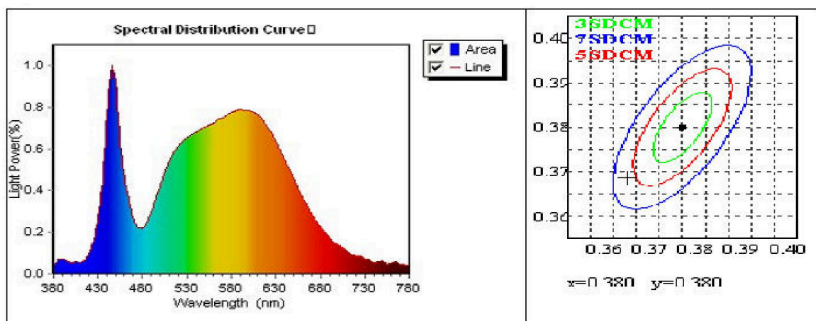
SDCM=5.6 SDCM Color Difference Chart
