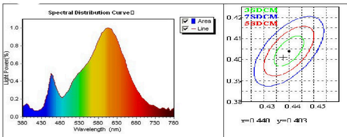
SDCM=1.4 SDCM Color Difference Chart
